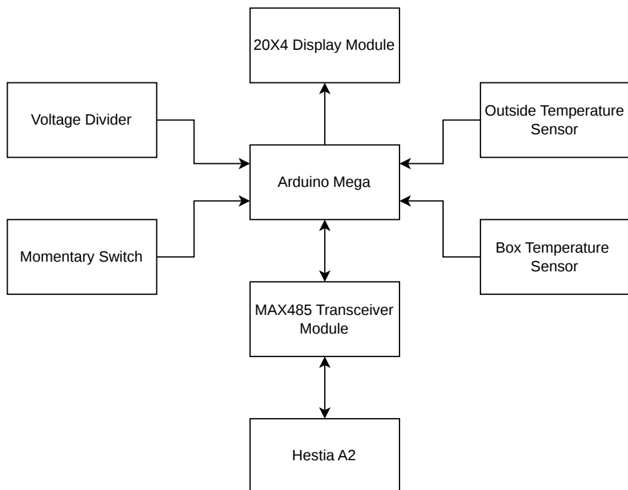
YT-011 Signal Path
