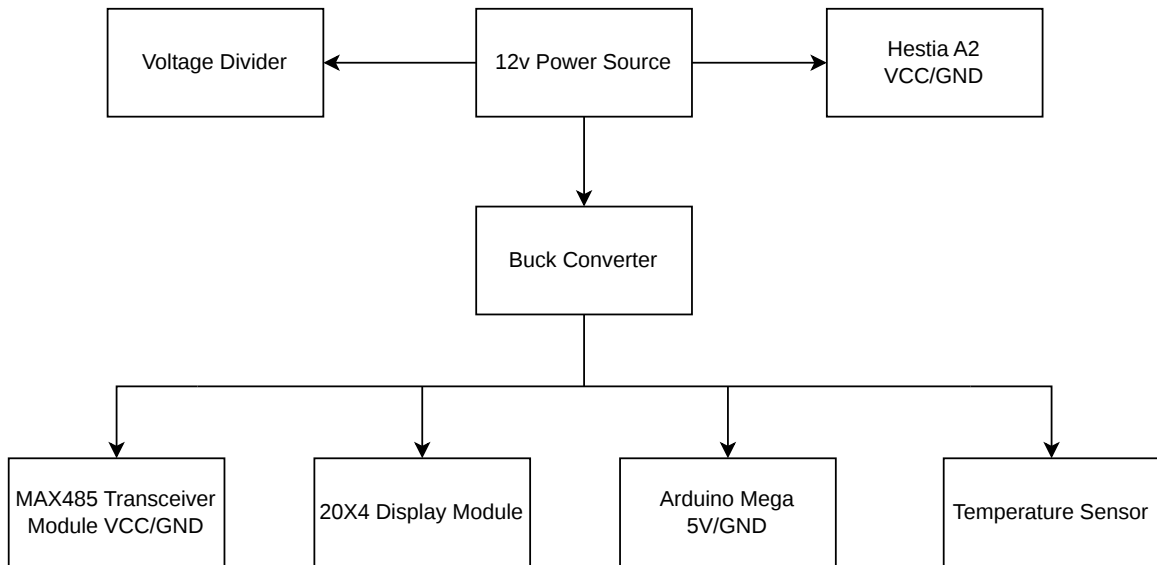
YT-011 Power Path
